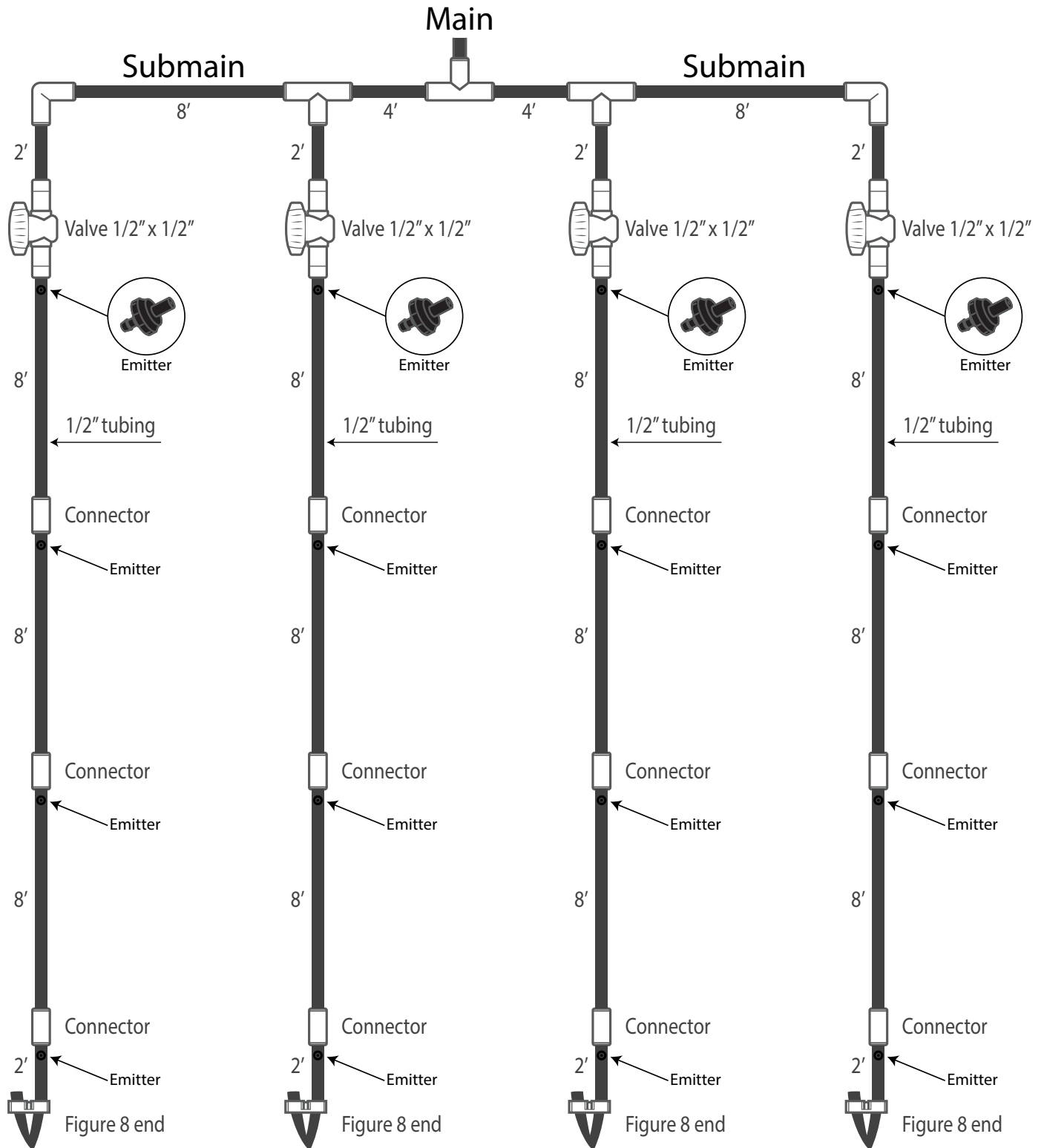
Figure 4: Lateral Components for a Drip Irrigation System
