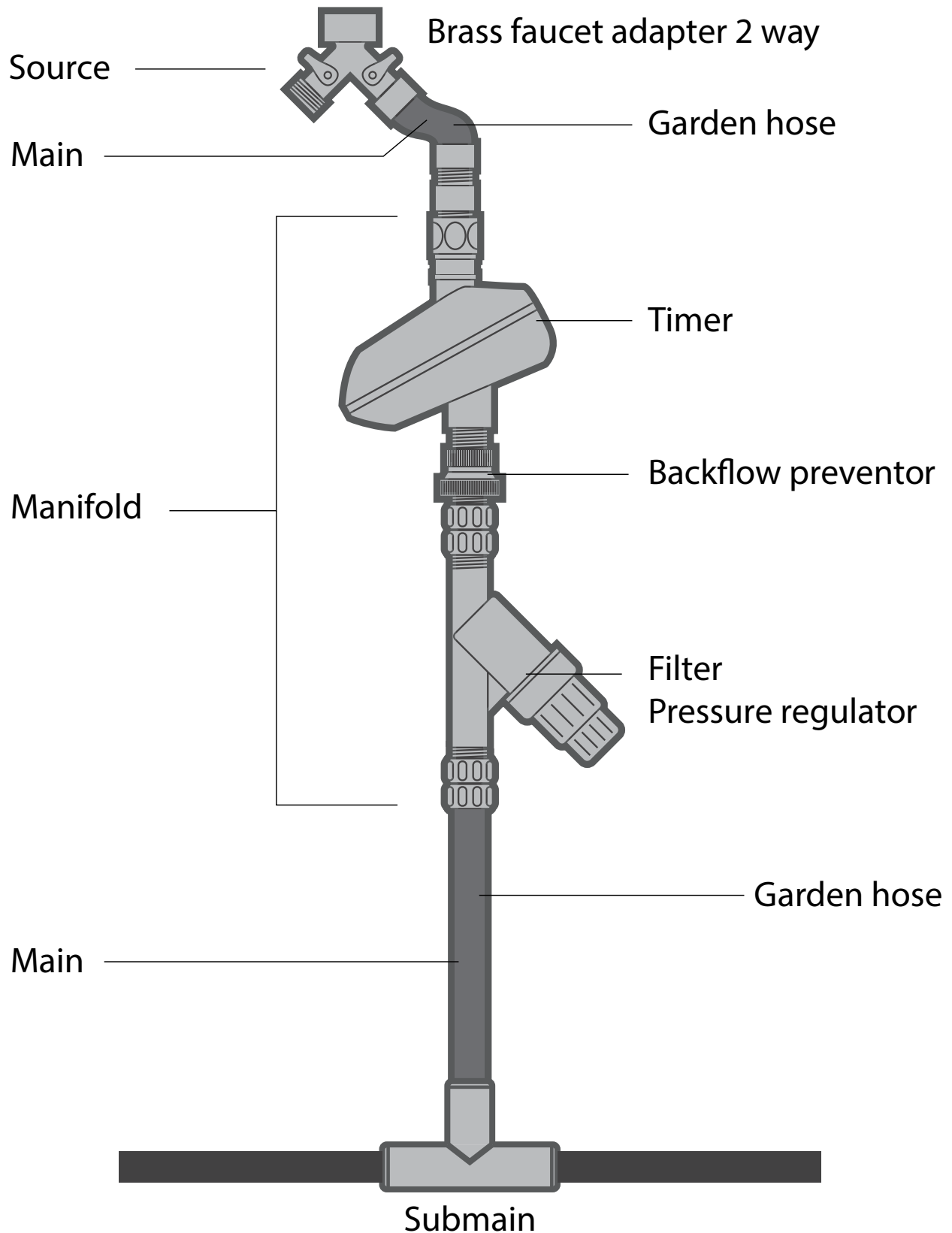
Figure 2: Main and Manifold Components for a Drip Irrigation System
